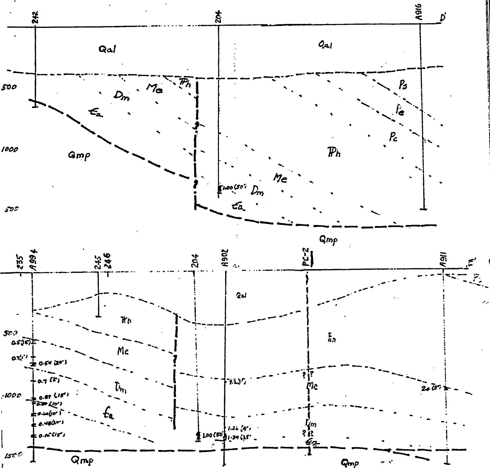
FIGURE 9: Interpretive Geological sections in area of 11-2.
